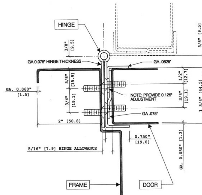
FULL WRAP EDGE GUARD (EDGE MOUNT)
