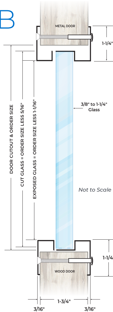
Door prep requires square cut corners
