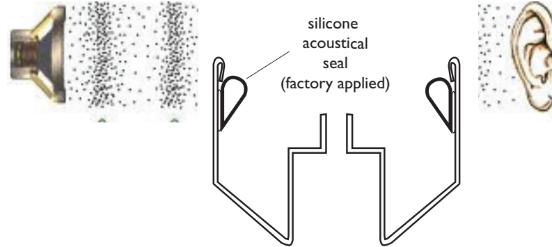
Silicone acoustical seal applied to reduce sound transmission
