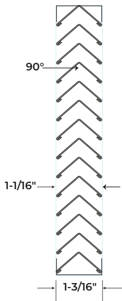
L-700-A-SS undersized 1/16" for clearance
