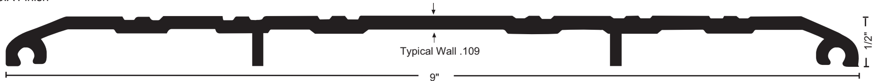
Type 4 For center hung single acting or double acting. Both ends mitered.
