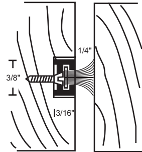
136P polypropylene pile 136PDKB Mortise dimensions 7/16" wide x desired depth. #2 SMS furnished.
